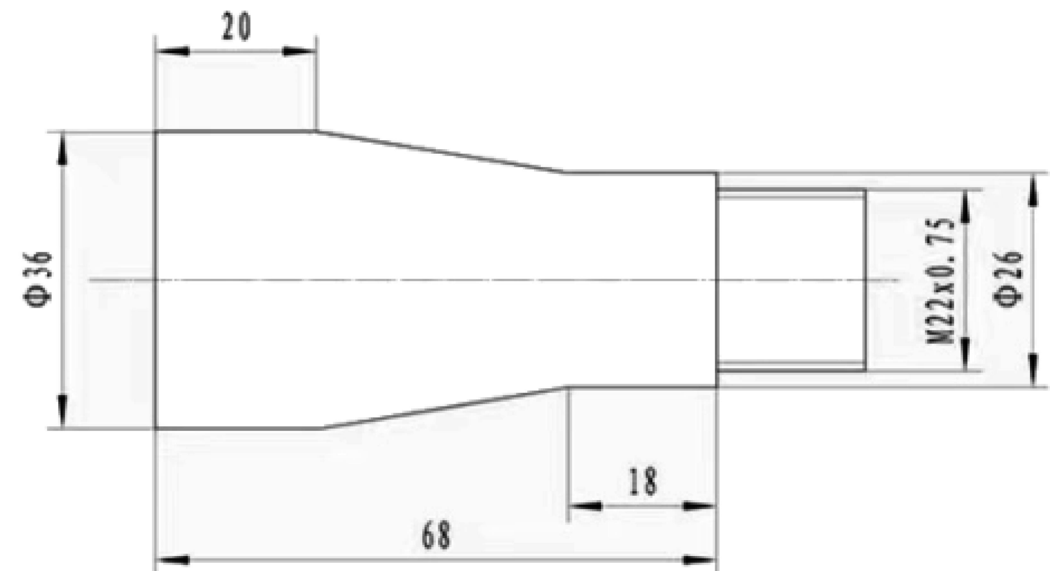
6x Beam Expander
