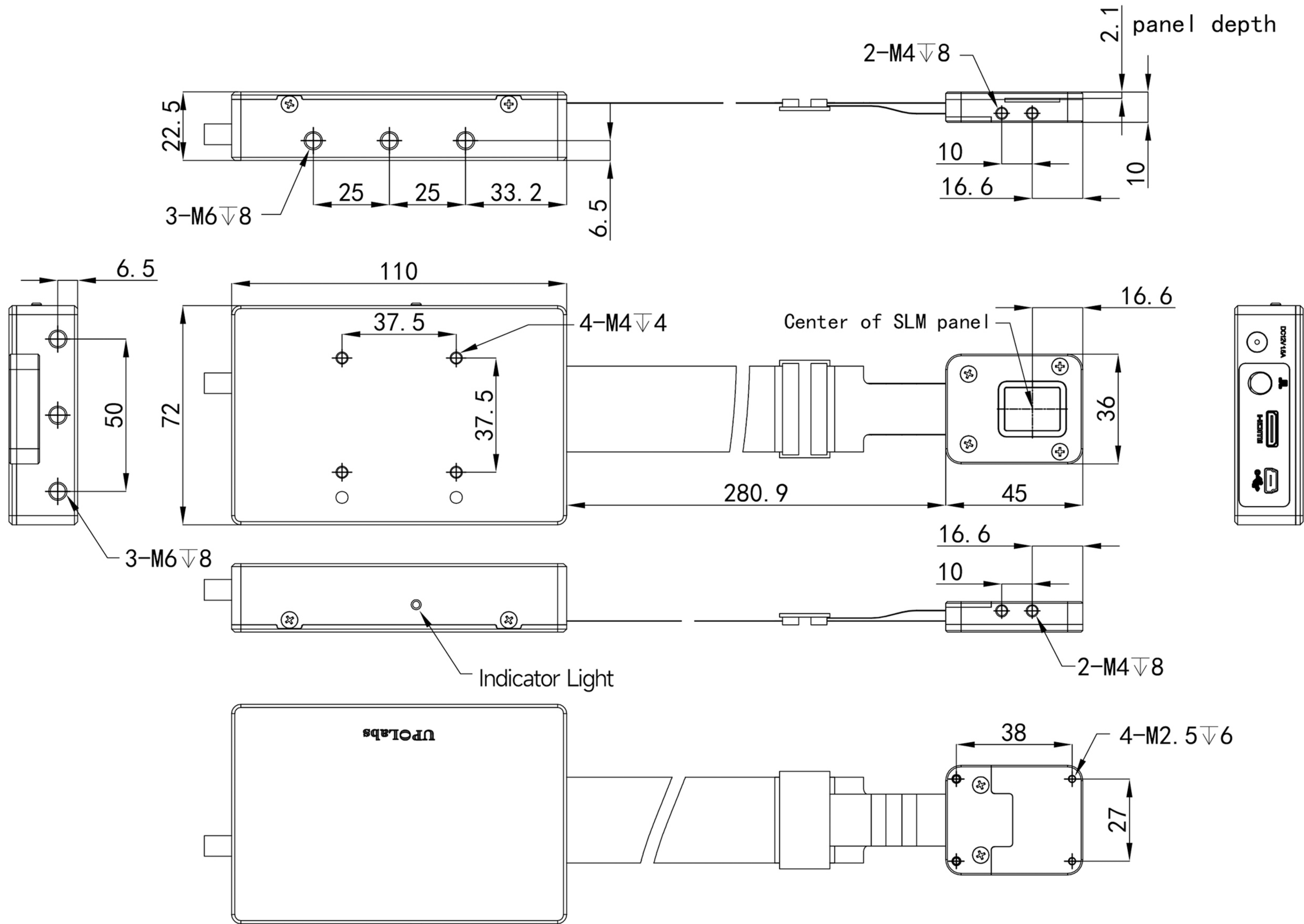
HDSLM80R Plus Split-type
